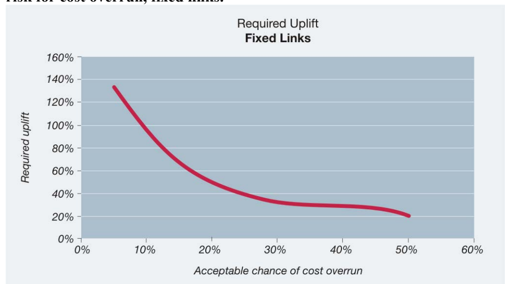
Figure 10 - Required uplift as function of the maximum acceptable level of risk for cost overrun, fixed links.
